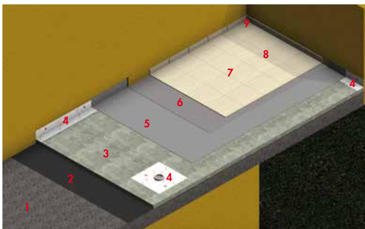
NEWLY BUILT TERRACES
