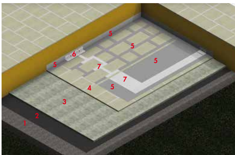
RESTORATION OF EXISTING TERRACE
