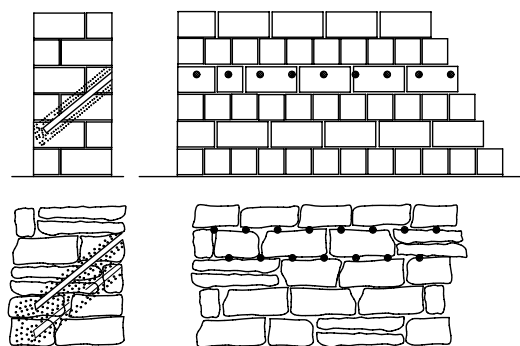
Example of bore hole arrangement – injection without pressure
